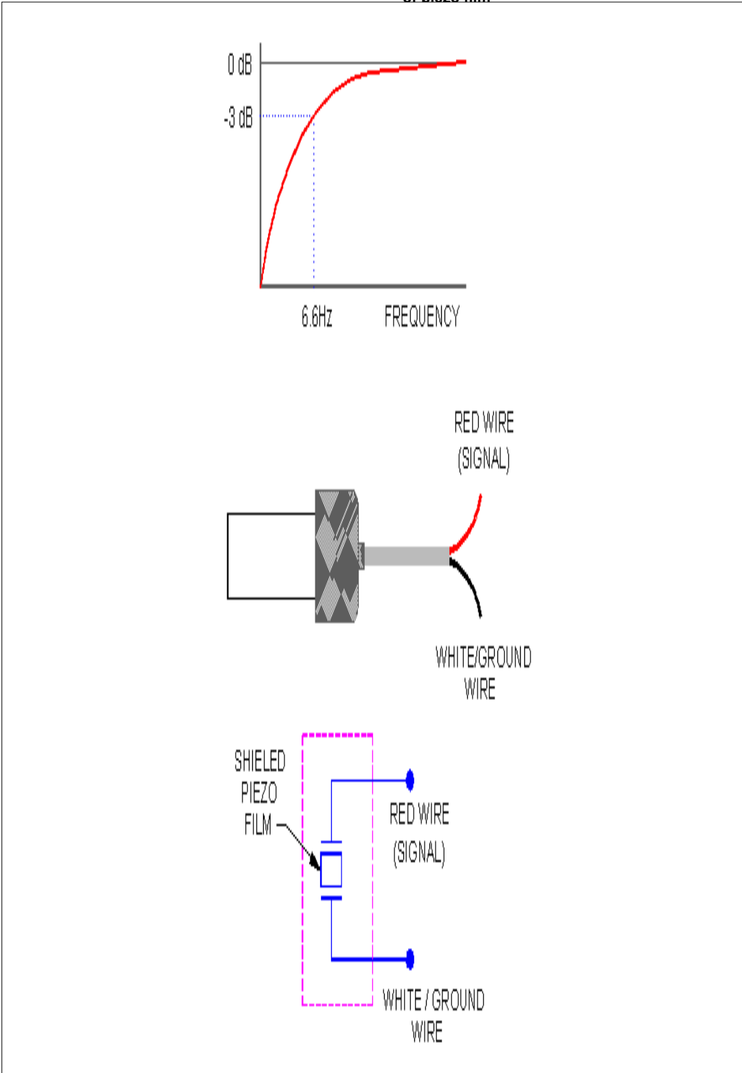
Figure 38. High pass filter characteristic of piezo film
