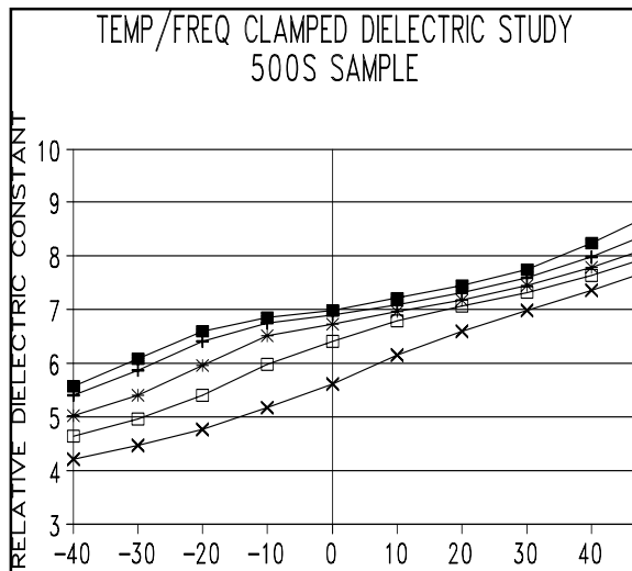
Figure 25b. Dielectric constant vs. temperature COPOLYMER
