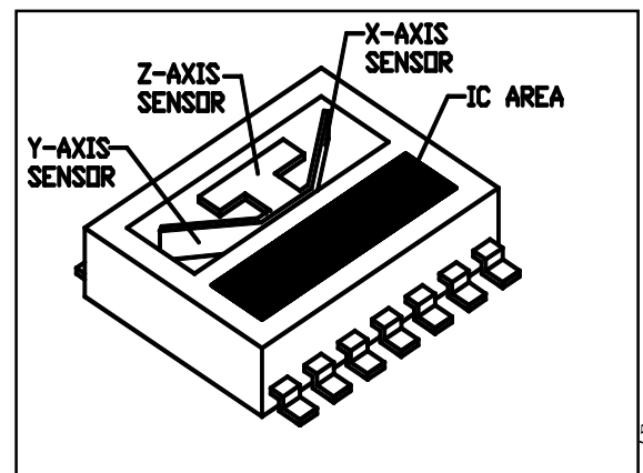
Figure 60. ACH-04-08-05 internal view
