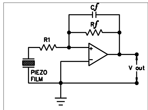
Figure 45. Op Amp Interface circuit acting as a charge amplifier
