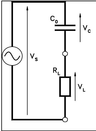
Figure 14. Potential divider
