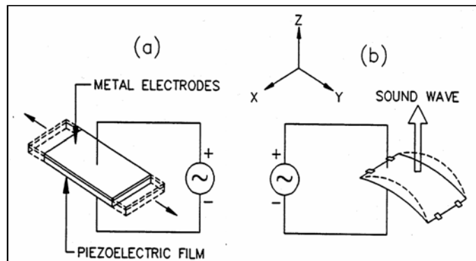
Figure 10. Clamped film in d_{31} mode produces sound
