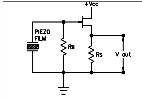
Figure 43. High frequency, low gain FET circuit interface
